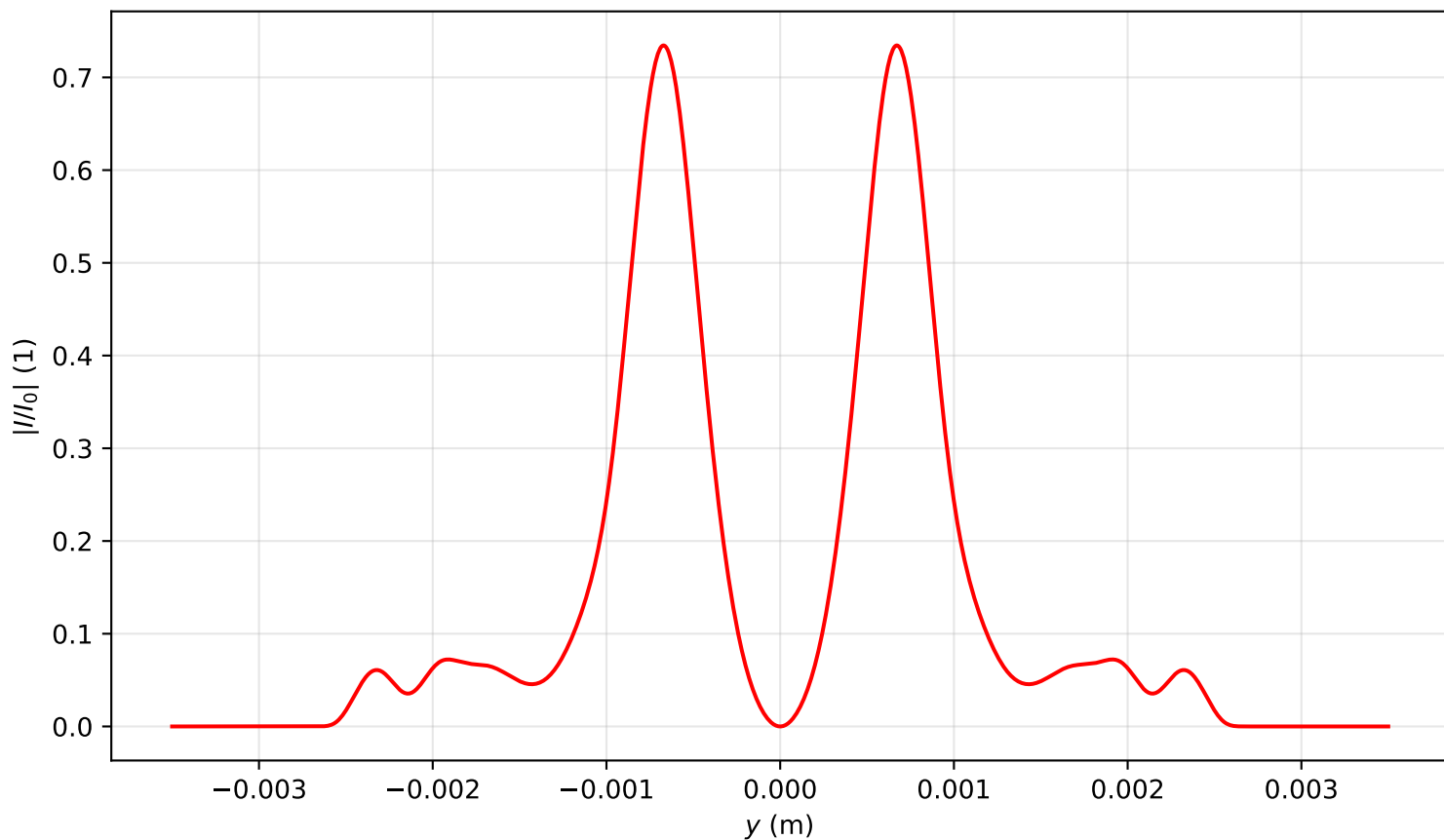
Intensity profile I(x=0, y, z=3.264)/I_0 , P_{in}=5.0P_{cr} , artificial time
